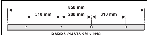
BARRA CHATA 3/4 x 3/16 3/4 x 3/16 Flat Bar | Barra Plana 3/4 x 3/16
